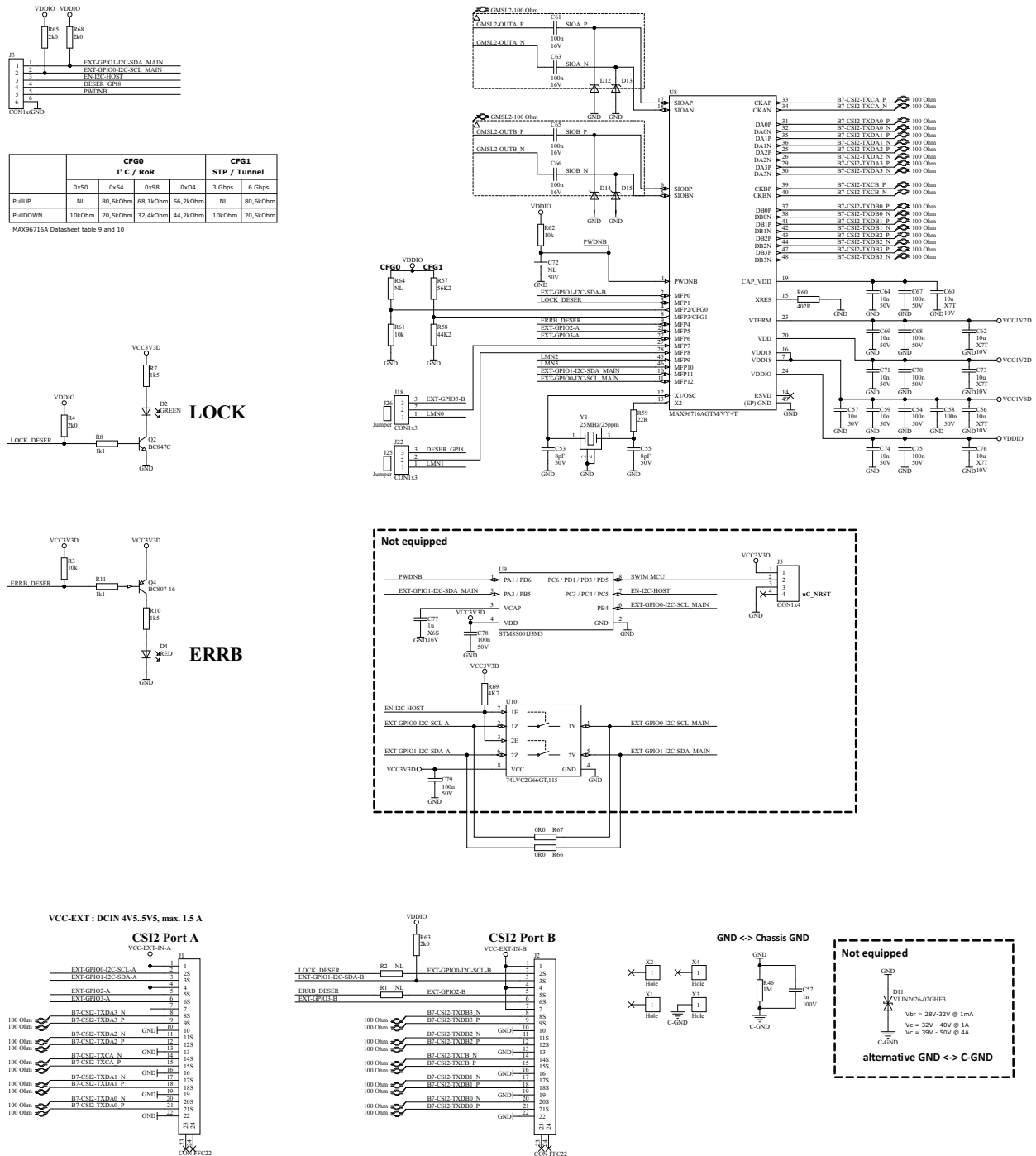
Figure 6: Deserializer Board GMSL2 STP to CSI-2 electronic schematics, part 1
