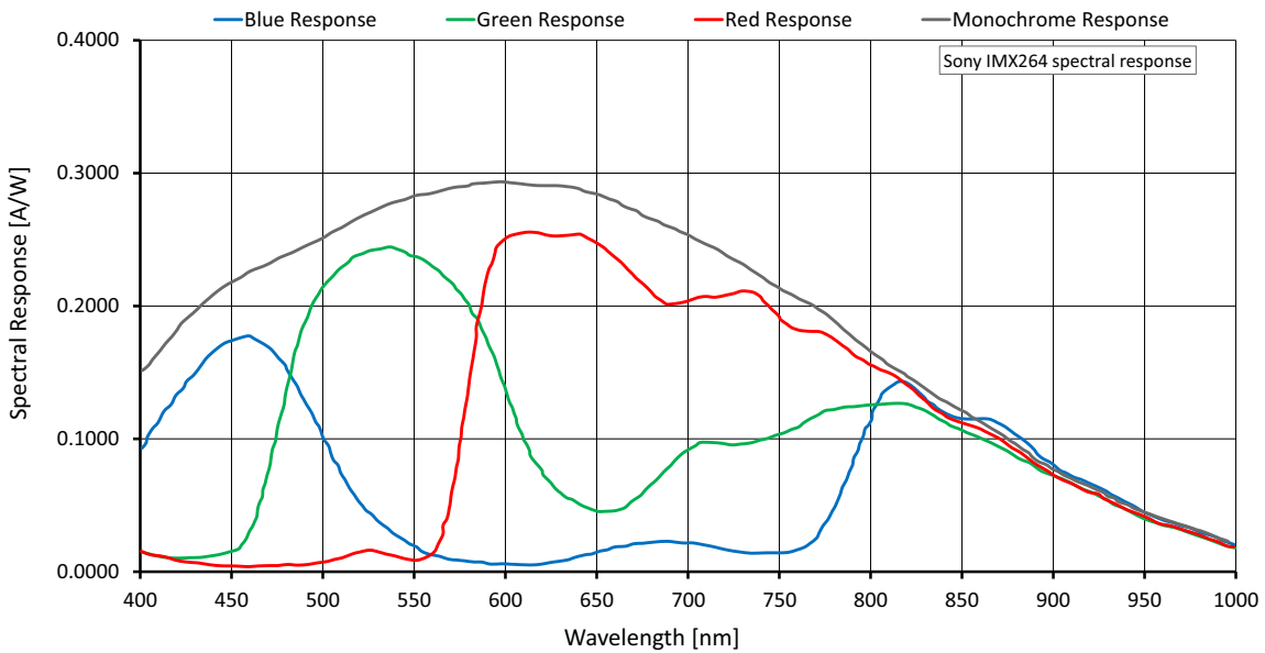
Figure 36: Mako G-507 (Sony IMX264) spectral response
