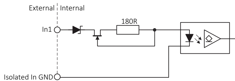
Figure 65: Input block diagram
