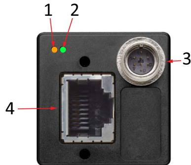
Figure 63: Rear view of Mako cameras
