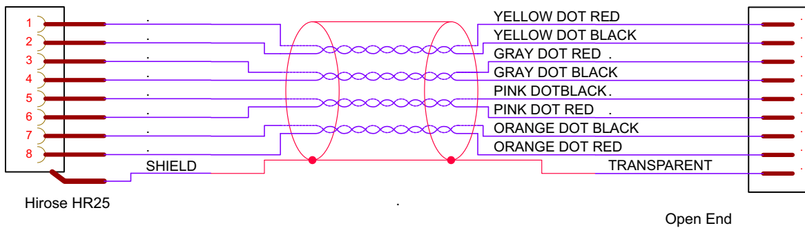
Figure 64: Mako cable color coding
